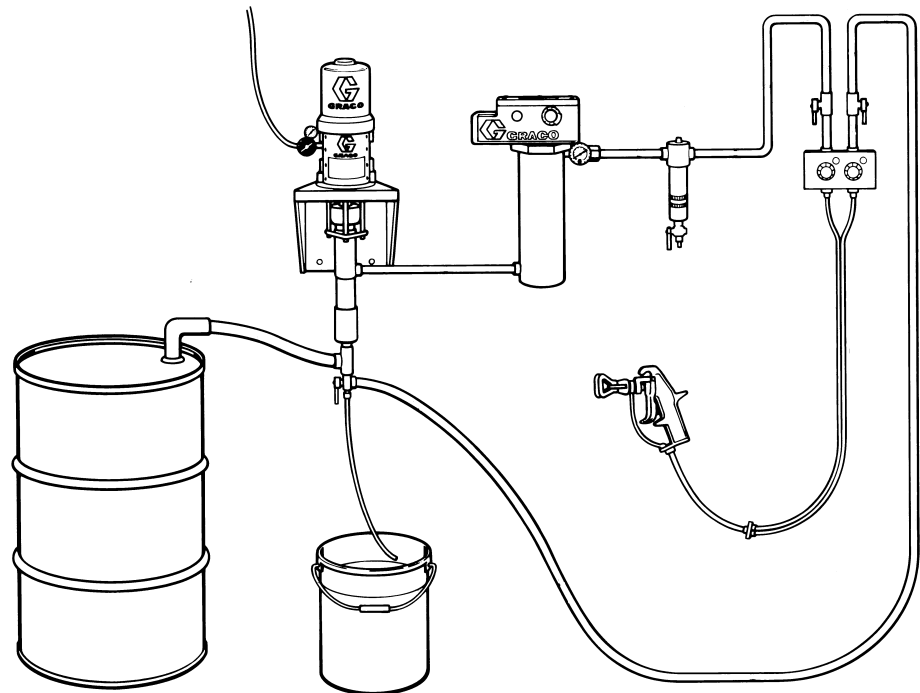
970-203 Manual Dispense Pump Package
